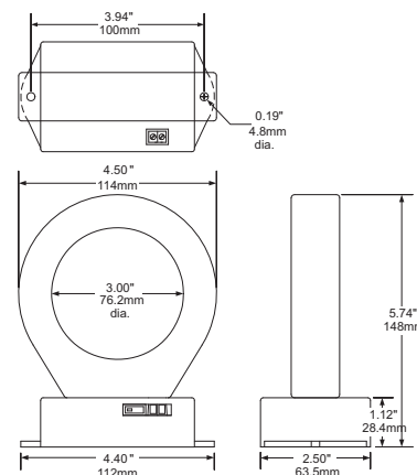
ACT Series 200 to 2000 Amp Fixed Core
