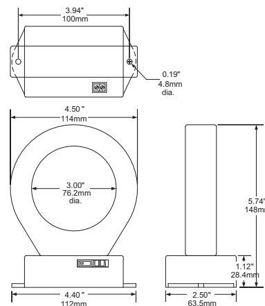
ACTR Series 200 to 2000 Amp Fixed Core
