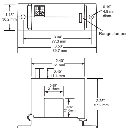
ACTR Series 2 to 200 Amp Split Core
